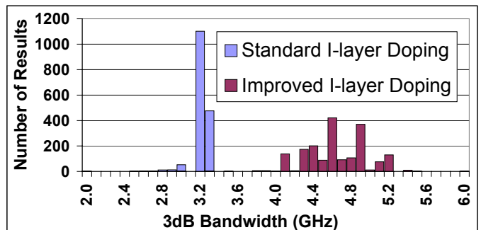
Histogram of 3 dB Bandwidth
