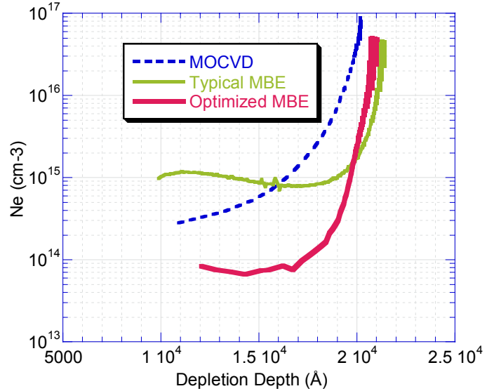
Corresponding N_e Profile from CV
