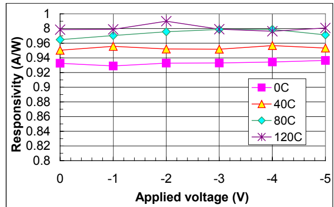
Photo Responsivity @ 1550 nm
