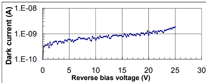
Dark Current
