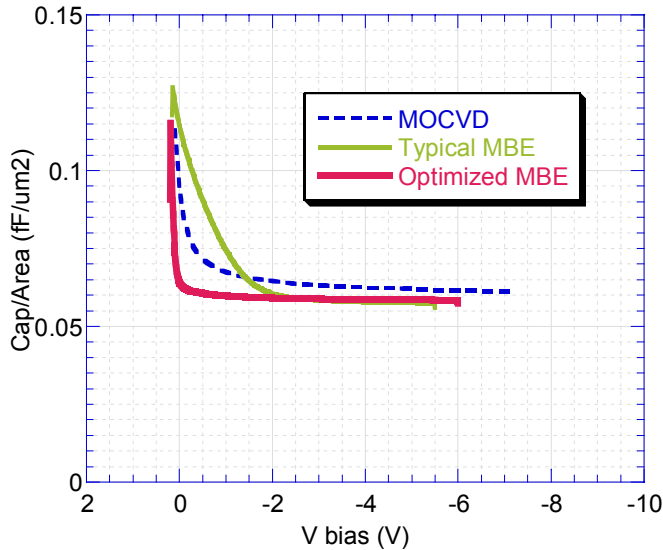
CV of PIN with 2 μm Intrinsic InGaAs
